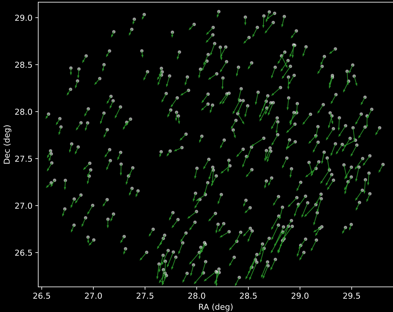
APOGEE DR17 Cluster 4 Proper Motion Vectors (n=299)
