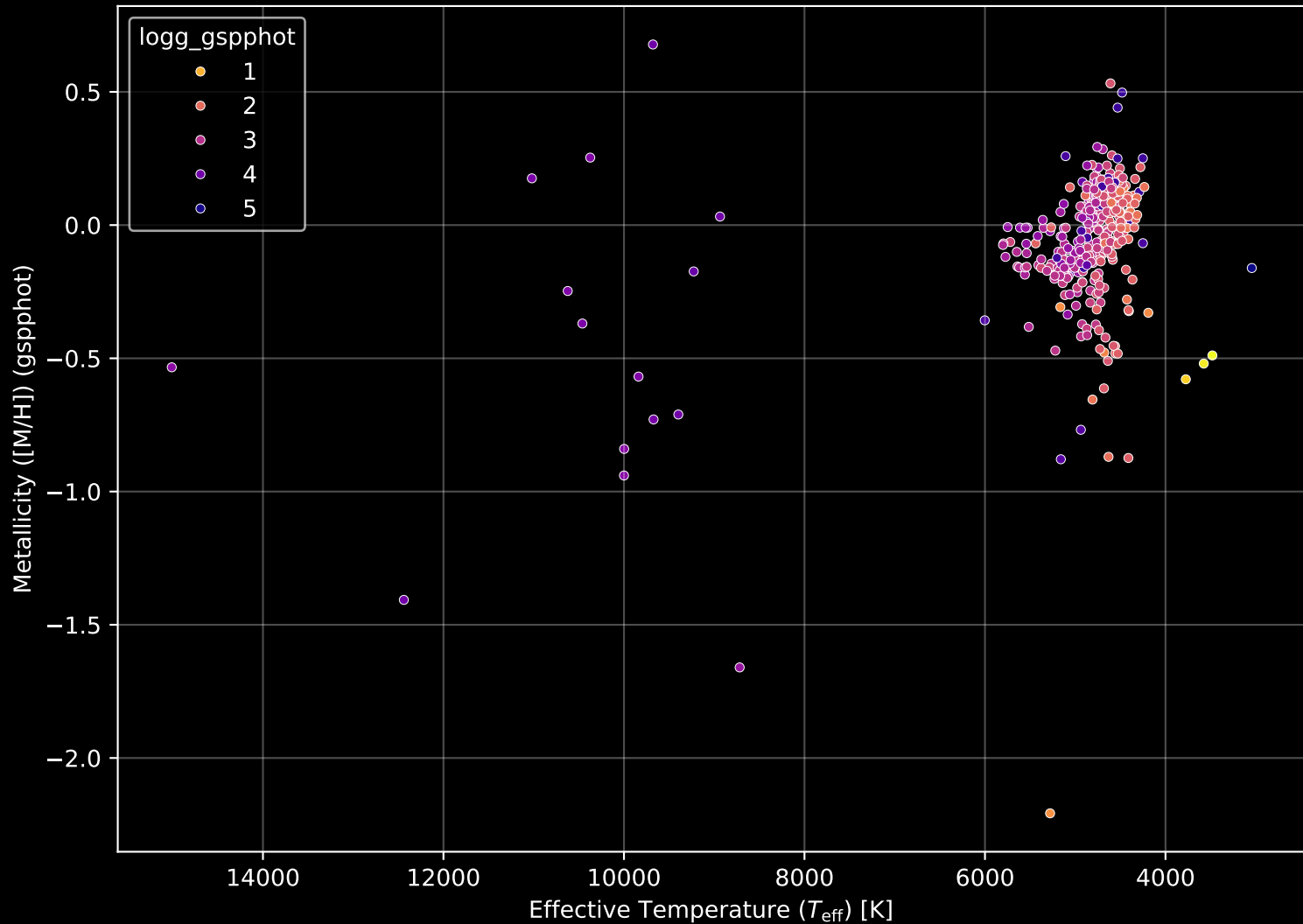
APOGEE DR17 Field: [060+08] Stellar Population Parameters (n= 415)
