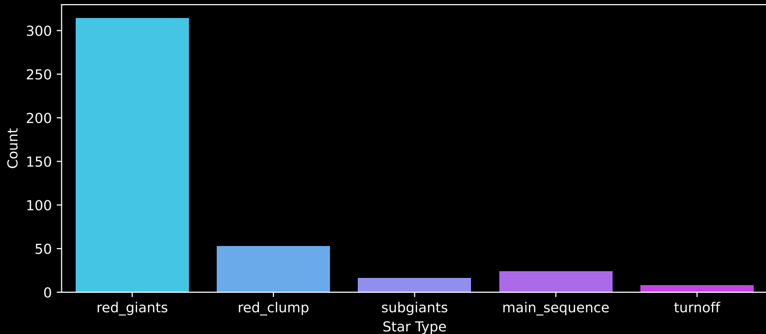
APOGEE DR17 Field: [060+08] Count plot of Star Type
