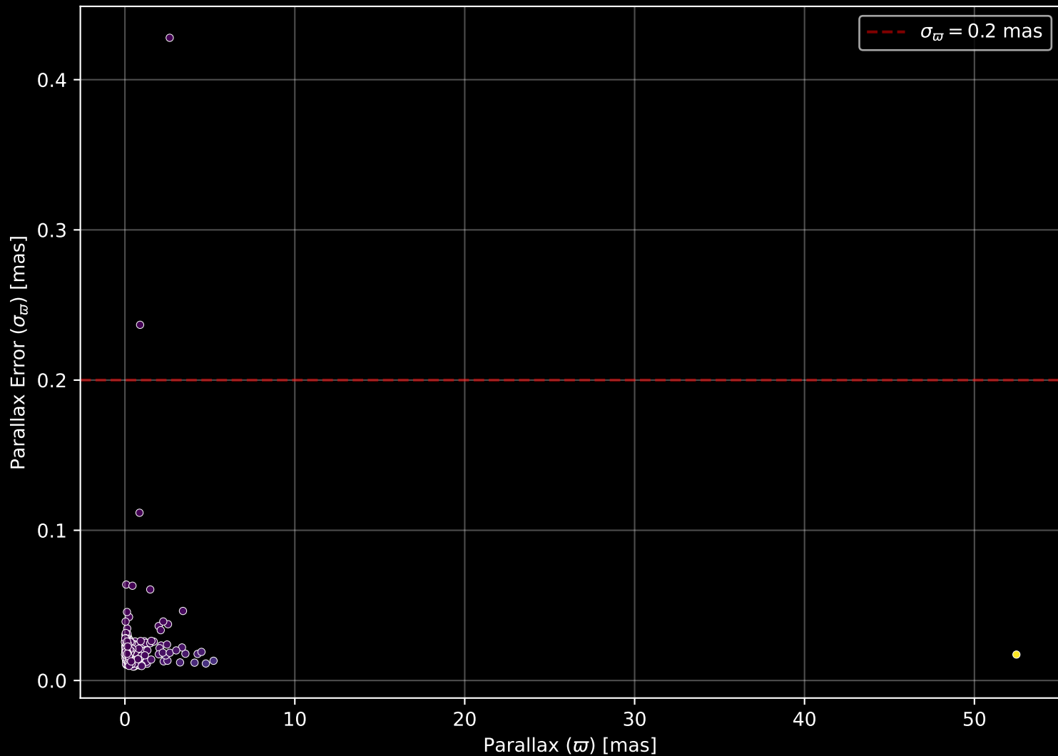
APOGEE DR17 Field: [060+08] Parallax Quality (n= 415)
