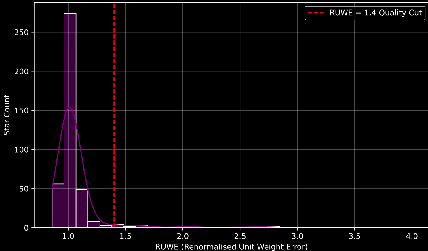
GAPOGEE DR17 Field [060+08] RUWE Distribution (n= 412)
