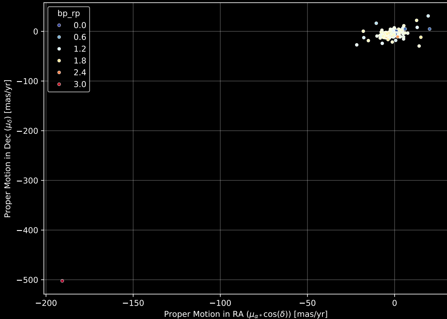
APOGEE DR17 Field: [060+08] Proper Motion Diagram (n= 415)
