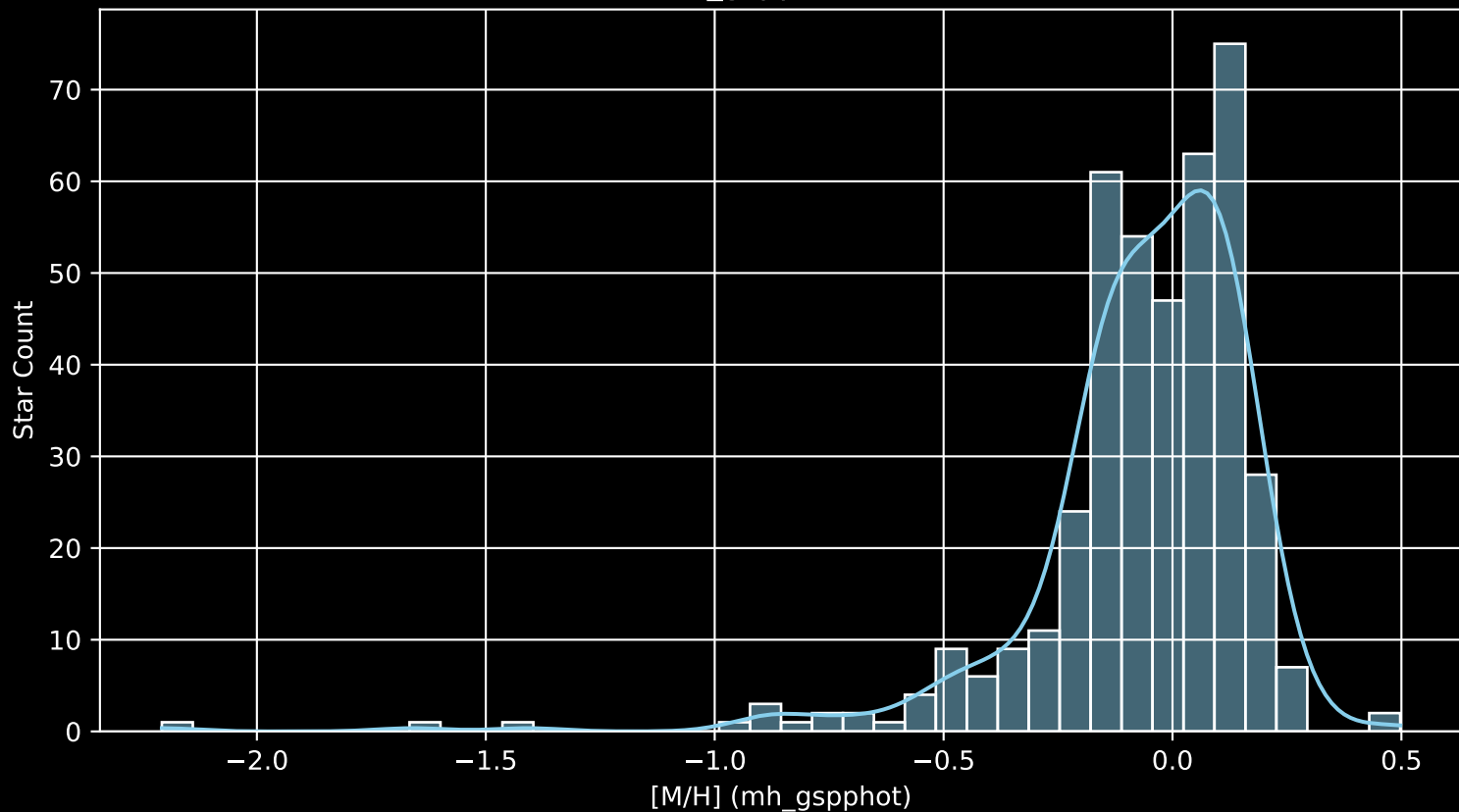
APOGEE DR17 Field: [060+08 [M/H] (mh_gspphot) (n= 413)
